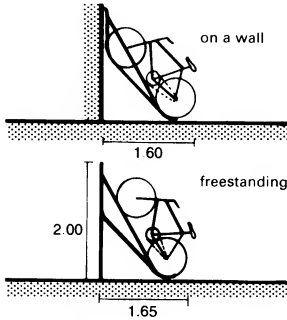
③ Tilted racks
